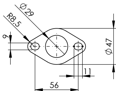
Flange s.s. sp.6mm "45B" cod.204392R
